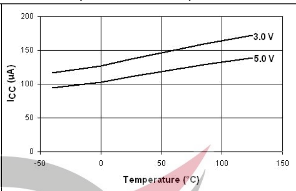
Figure 22. R_{ON} vs. temperature (STMP52141/2151)
