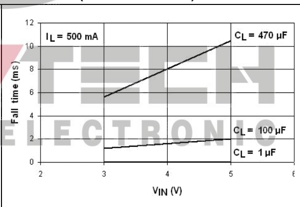
Figure 26. Output fall time vs. V_{IN} (STMP52141/2151)
